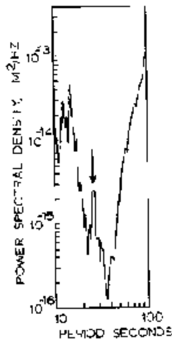
FIG. 1. Background earth motion recorded at ANMO showing a typical level of the 26-sec microseismic peak (arrow). Data from T, 15R, 04:23-30.
